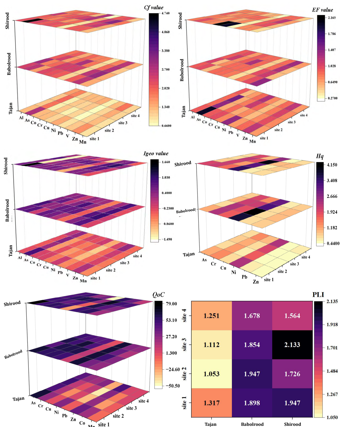
Figure 2) Spatial heatmaps of single indices for PTEs pollution in Tajan, Babolrood, and Shiroad Rivers; contamination factor ( C_f ), enrichment factor ( EF ), geoaccumulation index ( I_{geo} ), hazard quotient ( Hq ), quantification of contamination ( QoC ), and pollution load index ( PLI ).
