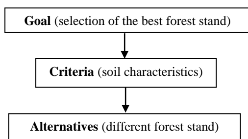
Figure 2 A schematic diagram of the AHP process
