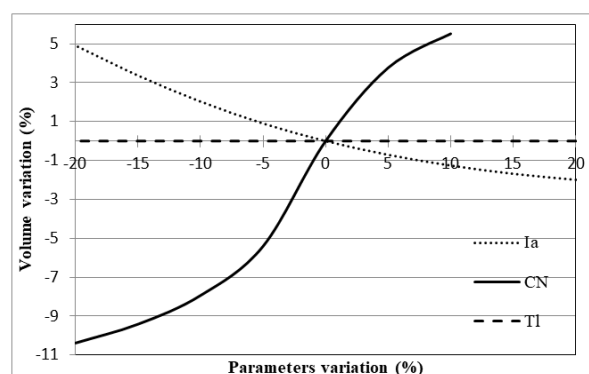
Figure 5) Sensitivity analysis results of HEC-HMS model.
