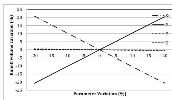
Figure 8) Sensitivity analysis of the water balance model.
