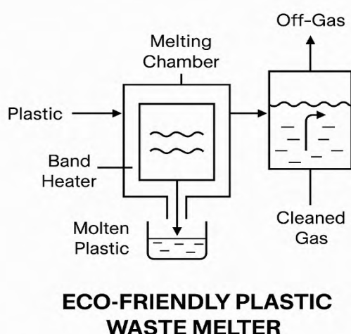
Figure 1) The air cleaner with a water bath system.
