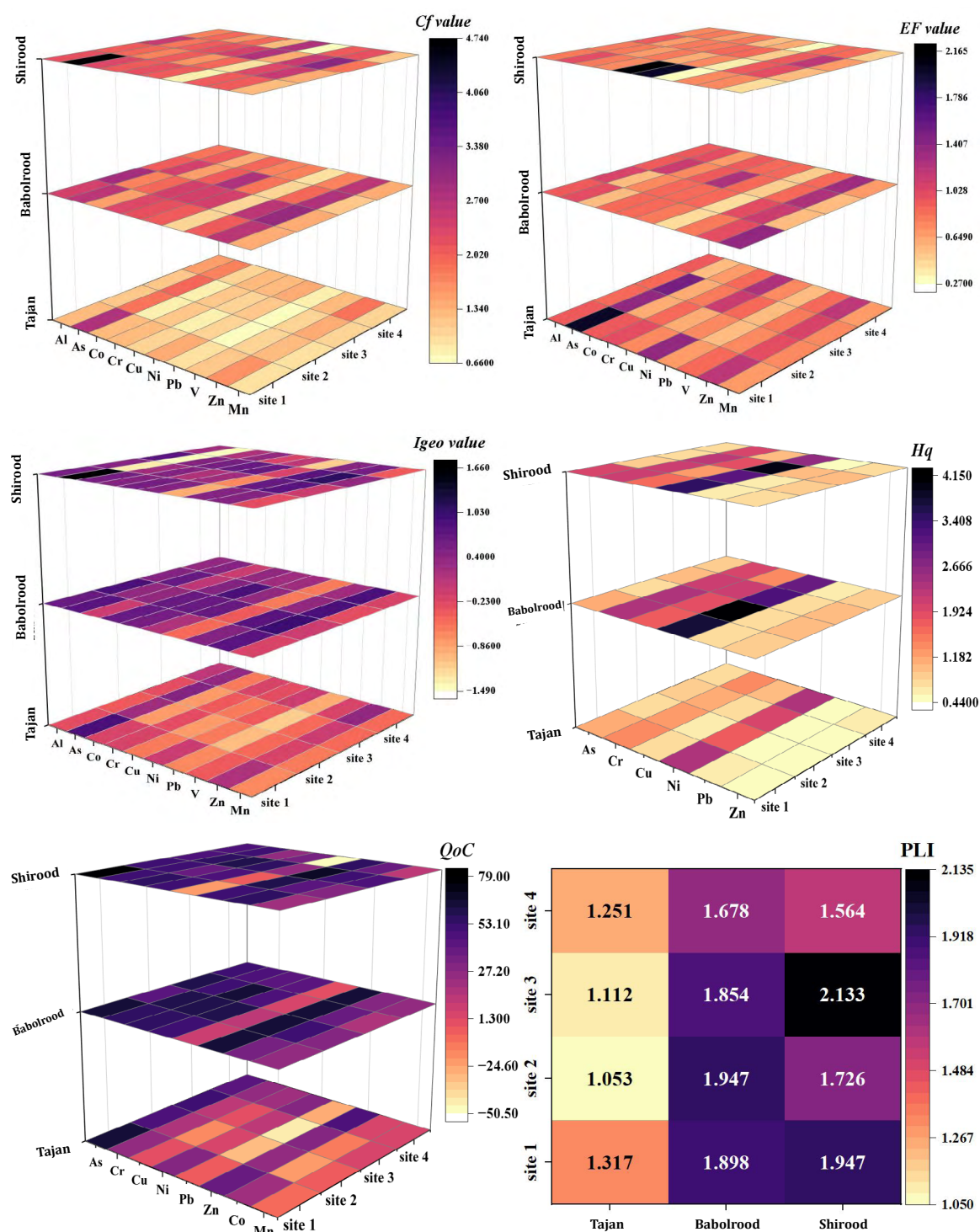
Figure 2) Spatial heatmaps of single indices for PTEs pollution in Tajan, Babolrood, and Shirood Rivers; contamination factor ( C_f ), enrichment factor ( EF ), geoaccumulation index ( I_{geo} ), hazard quotient ( Hq ), quantification of contamination ( QoC ), and pollution load index ( PLI ).
