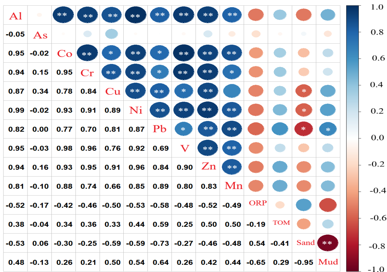
Figure 4) PCC matrix between PTEs and the general characteristics of sediments in the Babolrood, Tajan, and Shirood Rivers.
