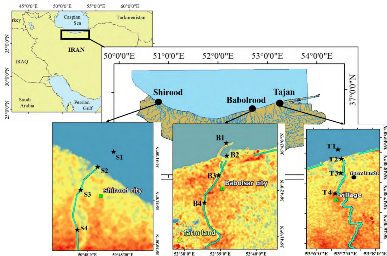
Figure 1) Map showing geographical coordinates of the sampling locations in the southern Caspian Sea, Tajan River (T1, T2, T3, T4), Babolrood River (B1, B2, B3, B4), and Shirood River (S1, S2, S3, and S4).
