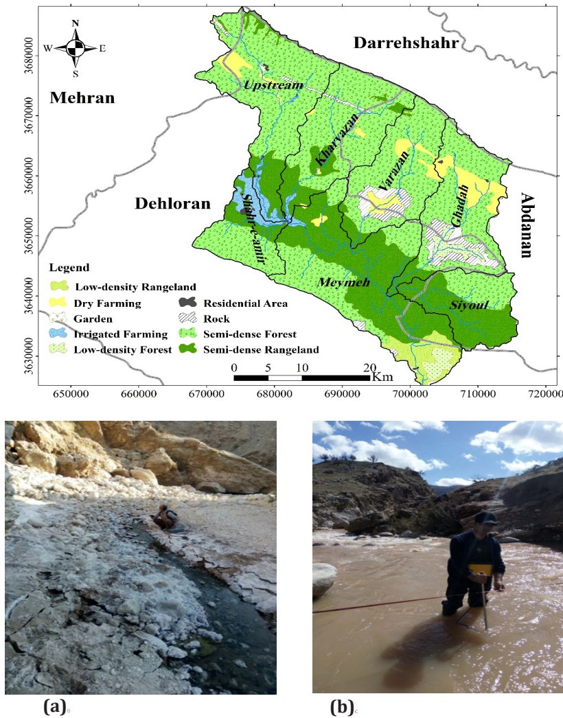
Figure 2) A scheme of the land uses and sub-watersheds in the Meymeh Watershed, with pictures from the field surveys. (a) refers to the Siyoul salty sub-watershed, where salt deposits are visible on the surface and around the stream; (b) refers to the main river at site 13.
