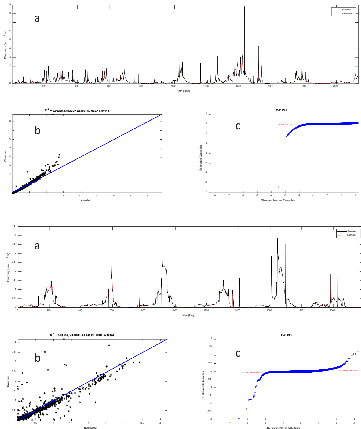
Figure 7) The results of EEMD-CNN runoff modeling, I) Kasilian Watershed, and II) Bar-Erich Watershed.
