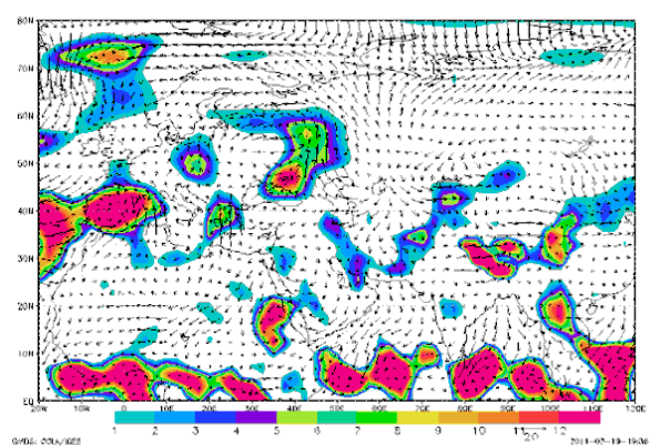
Figure 3 MFC map (1000 hPa) in SLP pattern 1 in dusty days
