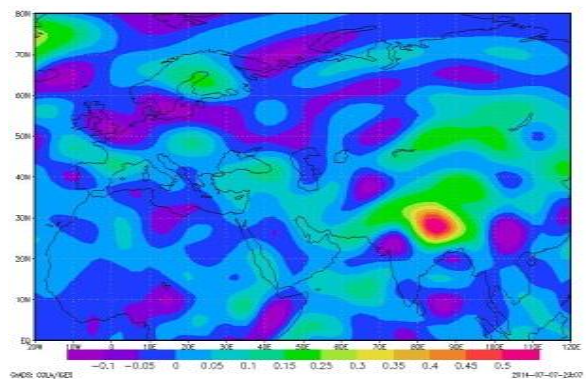
Figure 13 Omega map (1000 hPa) in SLP pattern 3 in dusty days
