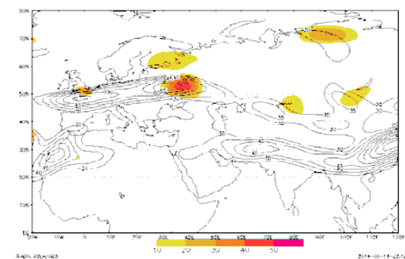
Figure 4 Jet stream map (300 hPa) in SLP pattern 1 in dusty days
