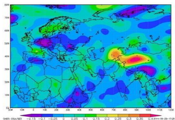
Figure 9 Omega map (1000 hPa) in SLP pattern 2 in dusty days
