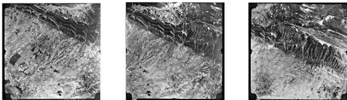
Figure 3 Aerial photographs depicting the glaciis of Sbeitla, Tunisia. Panchromatic B and W with Approx. Scale 1:25000; after Farshad, 1988.
