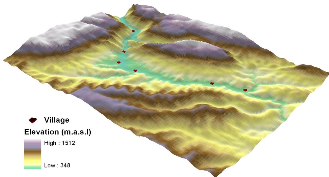
Figure 2 Topography of the study area (Source: USGS)
