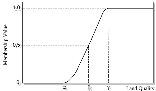
Figure 6 S membership function (adapted from Tang et al. , 1991)
