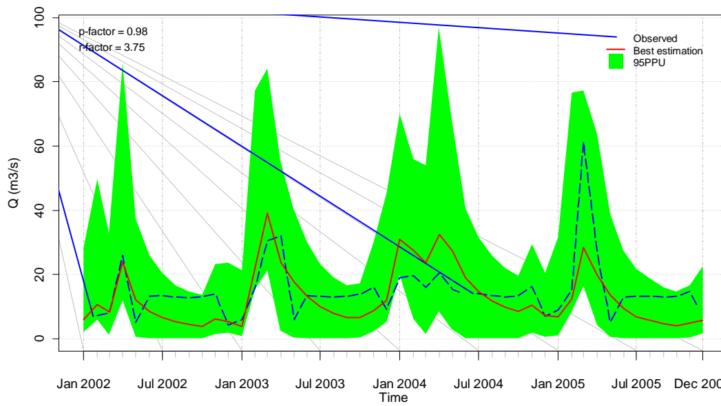
Figure 8 Observed and estimated mean monthly discharge at Polchehr station in validation period
