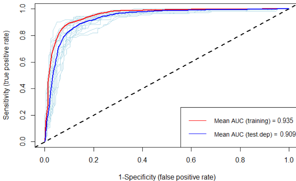
Figure 6 MaxEnt result: ROC curve for WSM
