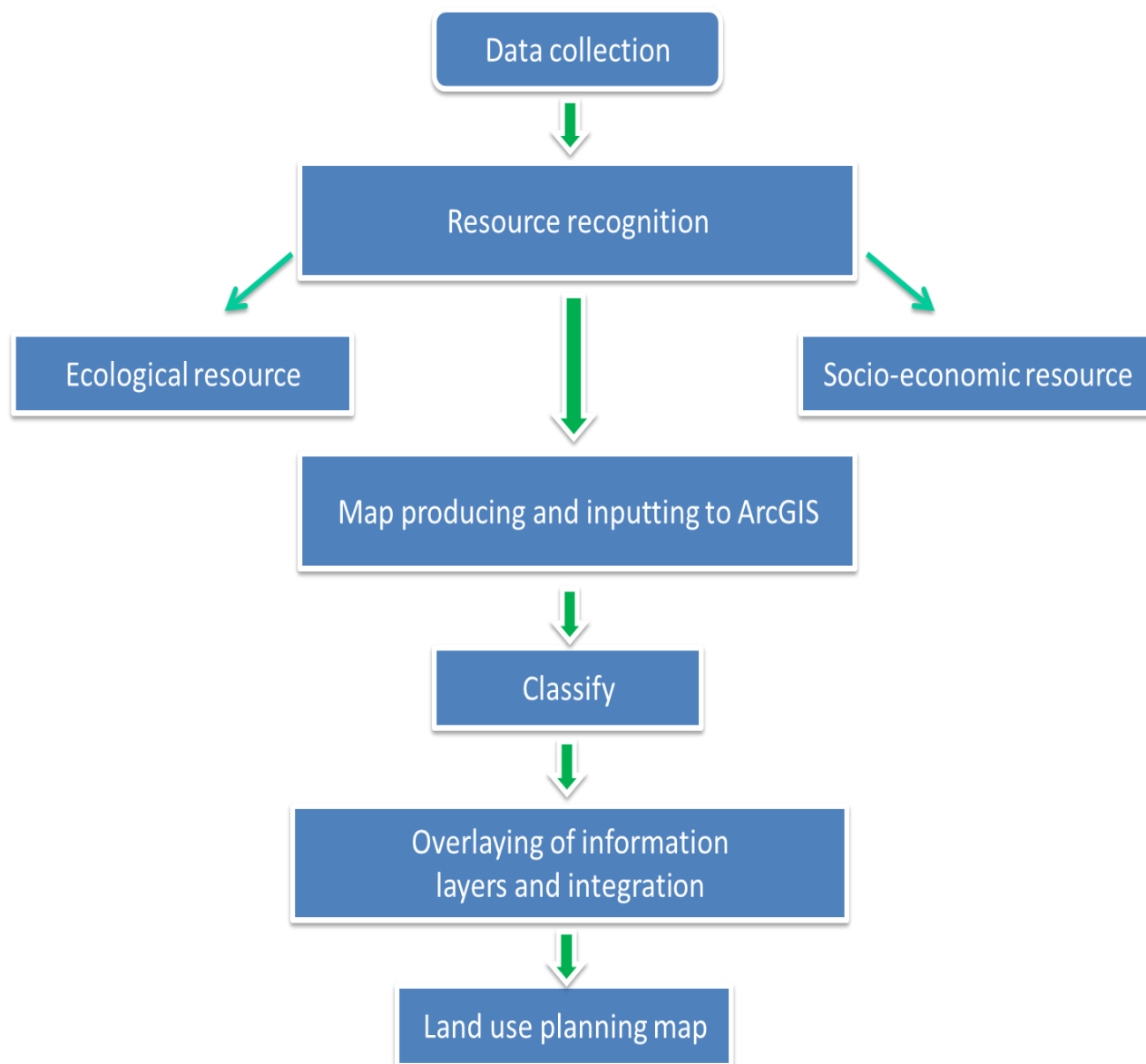
Figure 2 Flowchart showing the methodology for land-use planning adopted in the study
