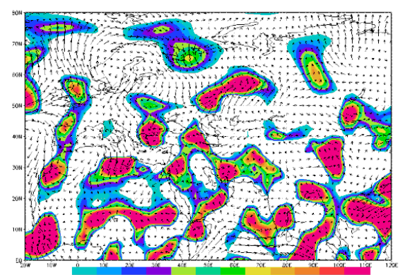
Figure 19 MFC map (1000 hPa) in SLP pattern 5 in dusty days
