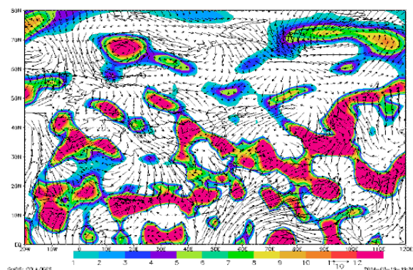
Figure 15 MFC map (1000 hPa) in SLP pattern 4 in dusty days
