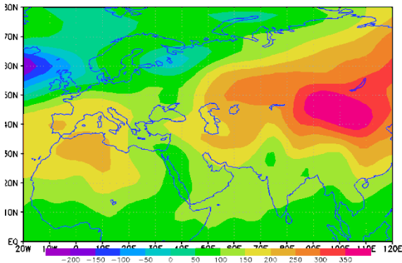
Figure 10 SLP pattern 3 map in dusty days
