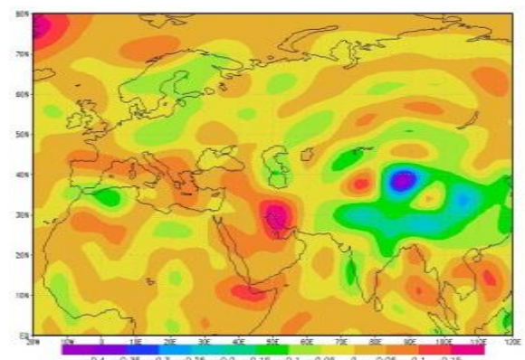
Figure 17 Omega map (1000 hPa) in SLP pattern 4 in dusty days
