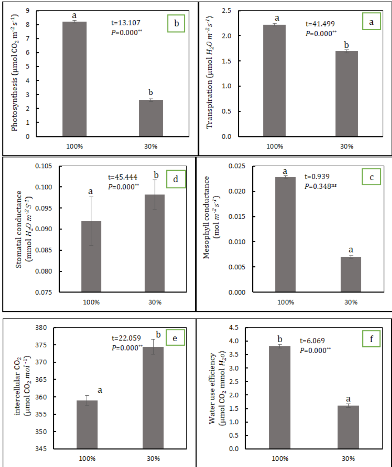
Figure 3) Comparison of gas exchange indices of common yew seedlings under drought stress.
