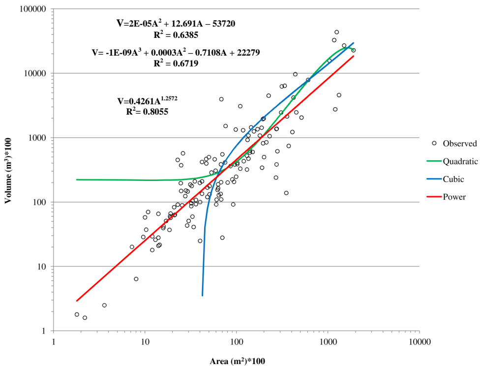
Figure 7 Logarithmic coordinate of the area-volume CE models after excluding the largest data
