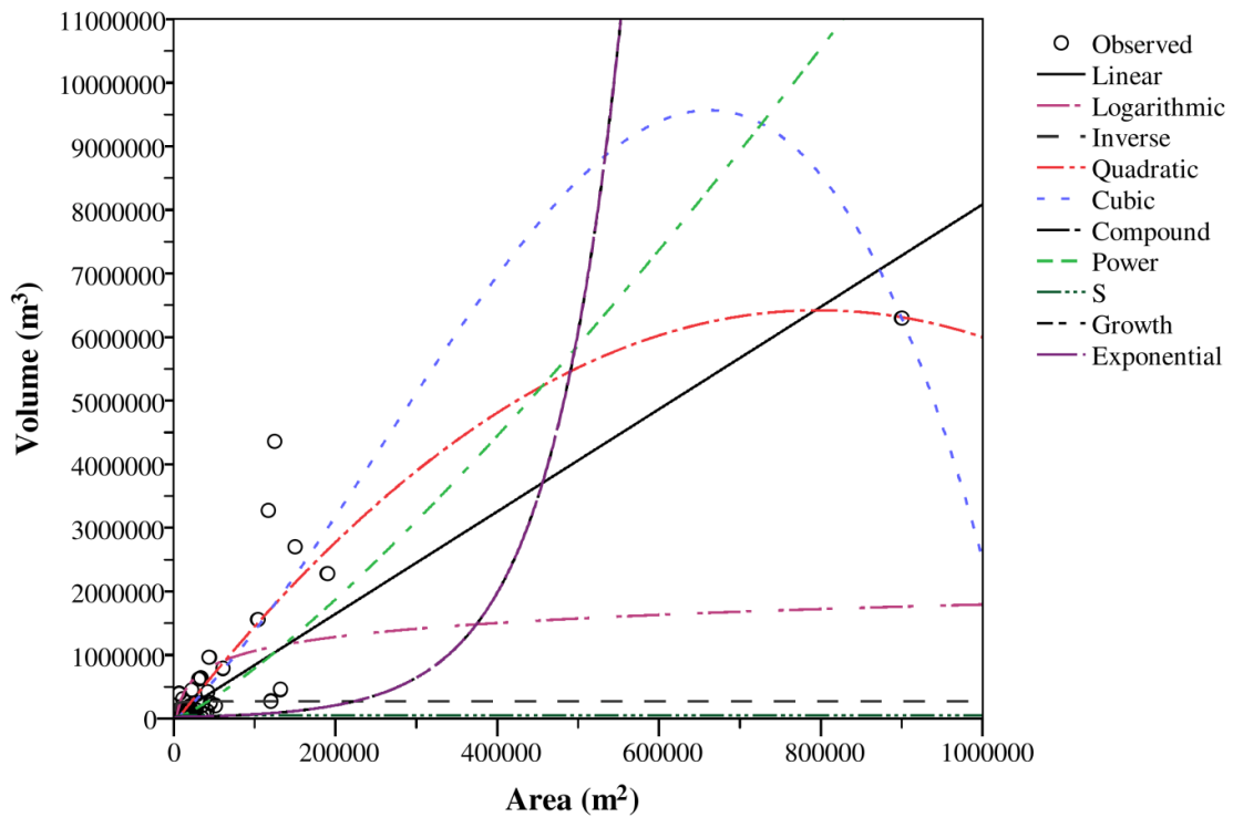
Figure 3 Scatter plot of the area-volume curve estimation models for the landslides of the study area
