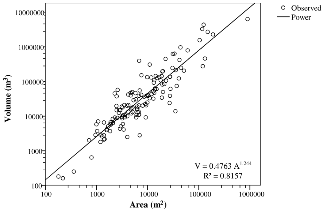
Figure 4 Logarithmic coordinate of the power law relationship between area (A) m 2 and volume (V) m 3 of the landslides in the study area
