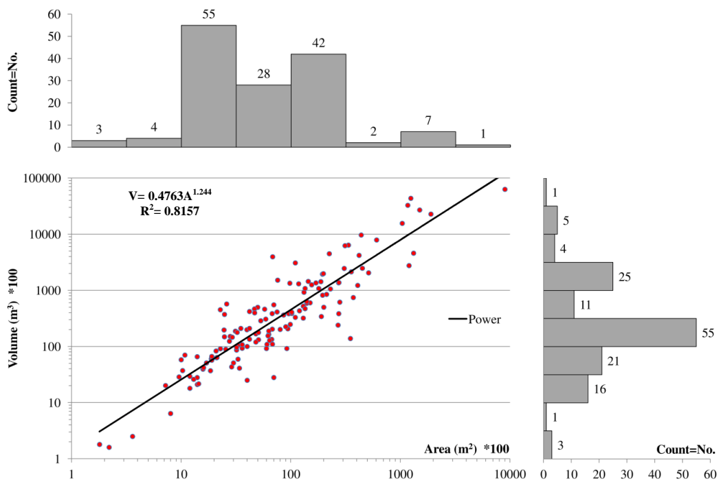
Figure 5 Frequency distribution of the landslides follows nearly a normal distribution related to their areas and volumes. Gray columns show the landslides frequency in different classes of the areas and volumes
