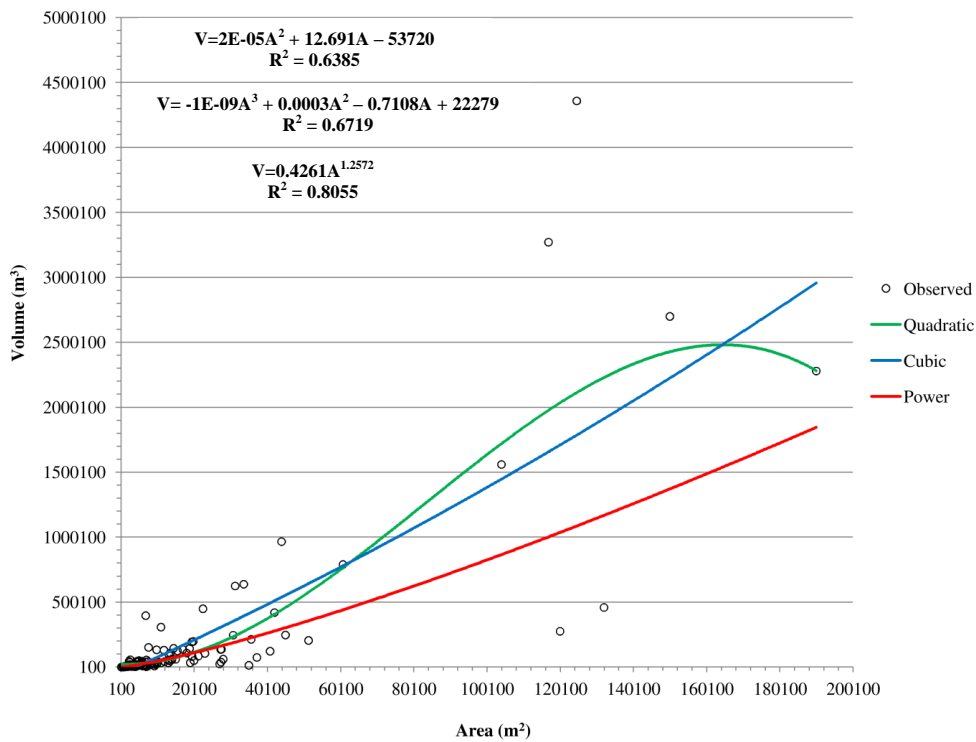
Figure 6 Area-volume power law, quadratic, and cubic models after excluding the largest data
